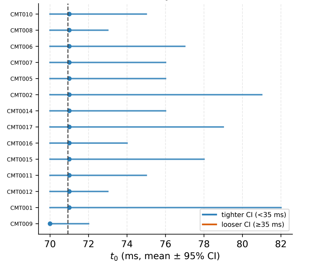
C. SRT non-decision time — estimated per participant (individual differences preserved; not floored)
