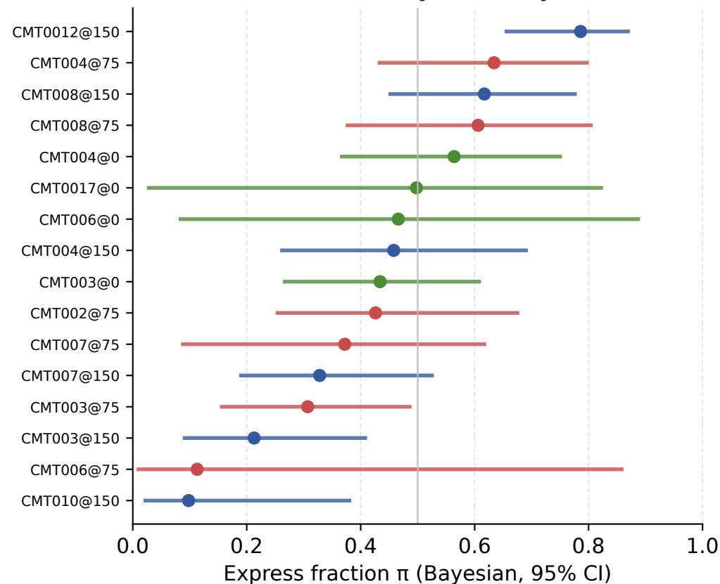
B. SRT express fraction & uncertainty (wide bars = bimodality not firmly identified)
