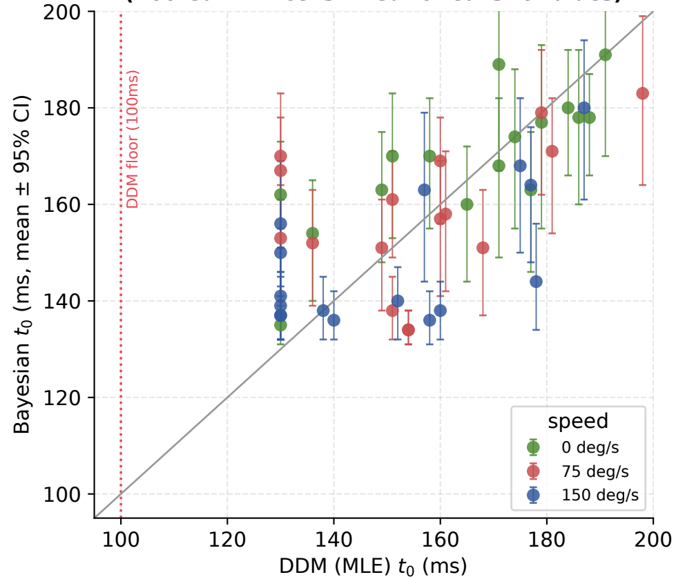
A. HRT: Bayesian resolves the floor degeneracy (floored DDM cells lifted to realistic values)
